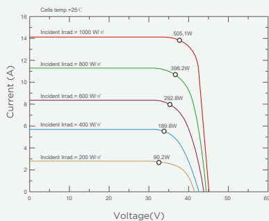
Current-Voltage Curve(SP505M-66H)
