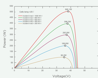
Power-Voltage Curve(SP505M-66H)
