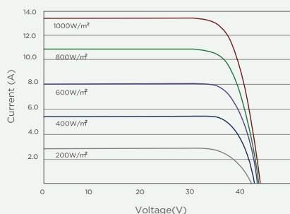
I-V CURVES OF PV MODULE(SP590M-60HB)
