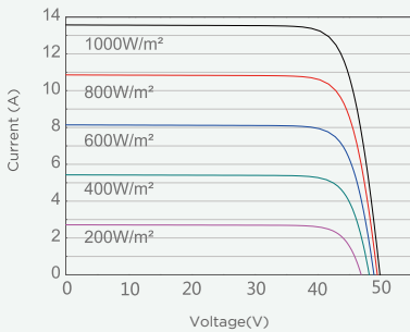
Current-Voltage Curve(SP540M-72HB)
