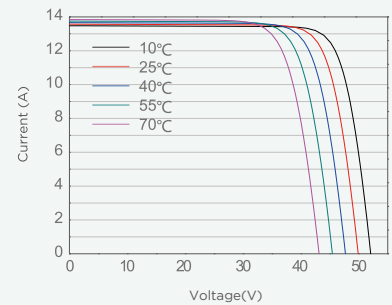
Current-Voltage Curve(SP540M-72HB)
