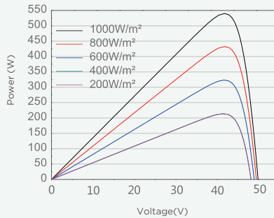
Current-Voltage Curve(SP540M-72HB)
