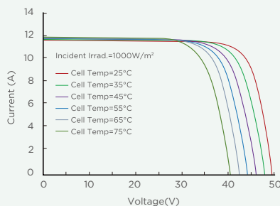
Current-Voltage Curve(SP440M-72HB)
