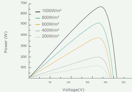
Current-Voltage Curve(660W)
