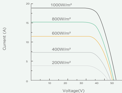
Current-Voltage Curve(660W)
