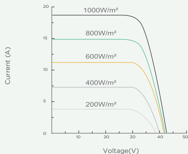
Current-Voltage Curve(605W)
